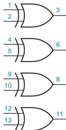
74x86
